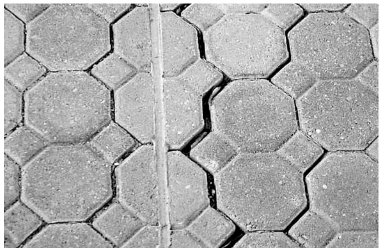
Figure 12. An absence of edge restraints and use of a sealant in this construction joint caused the pavers to shift and open their joints on both sides of the sealant.
