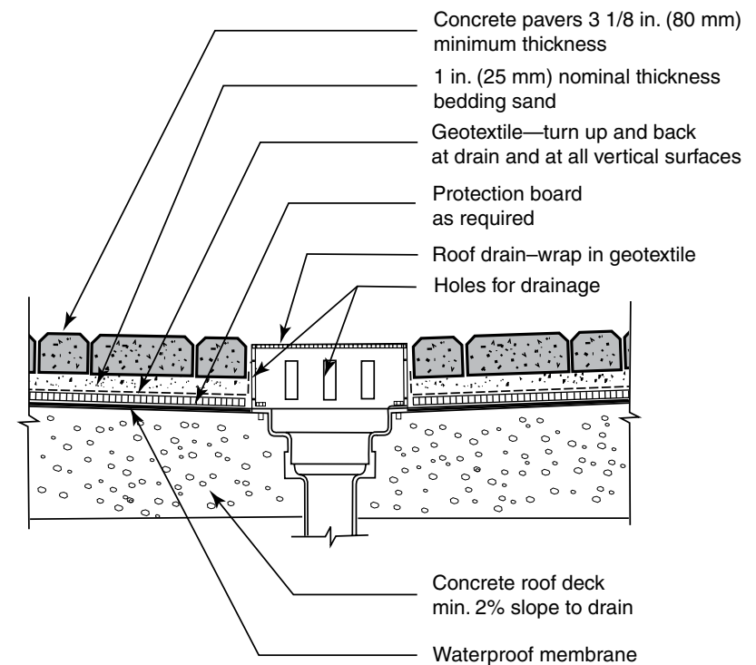
Figure 17. A drain detail on a vehicular roof application.
