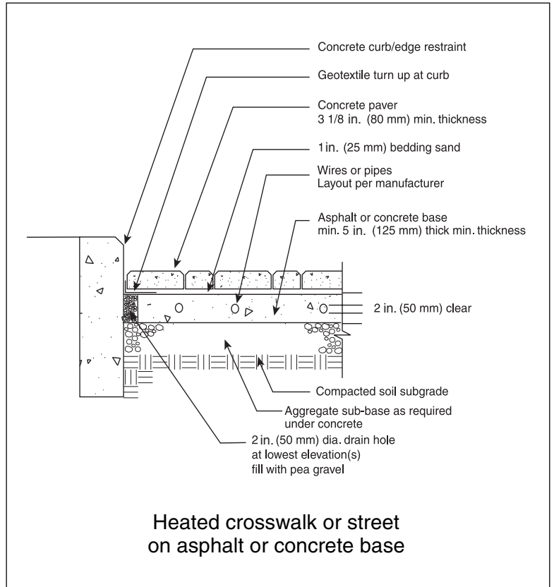
Figure 5. A typical cross section of a heated interlocking concrete pavement for crosswalks and roads subject to vehicular traffic.
