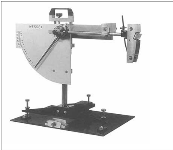
Figure 3. A British Pendulum Tester
